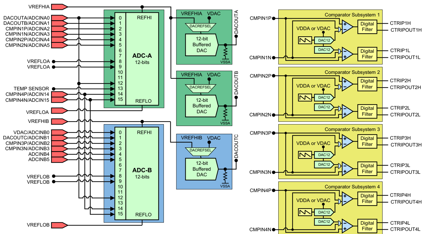
Figure 8-2. Analog Subsystem Block Diagram (100-Pin PZP)
