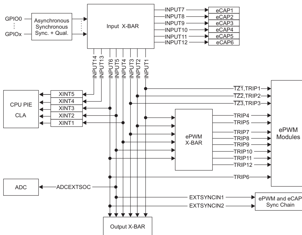
Figure 7-1. Input X-BAR
