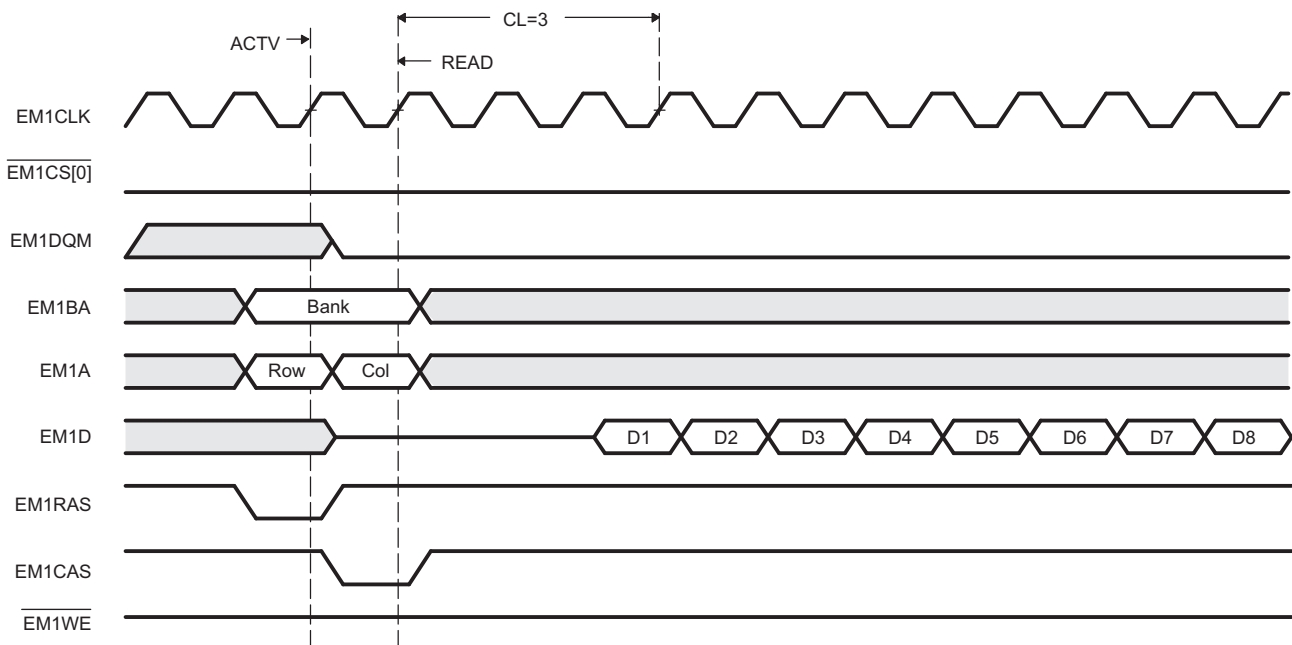
Figure 23-6. Timing Waveform for Basic SDRAM Read Operation
