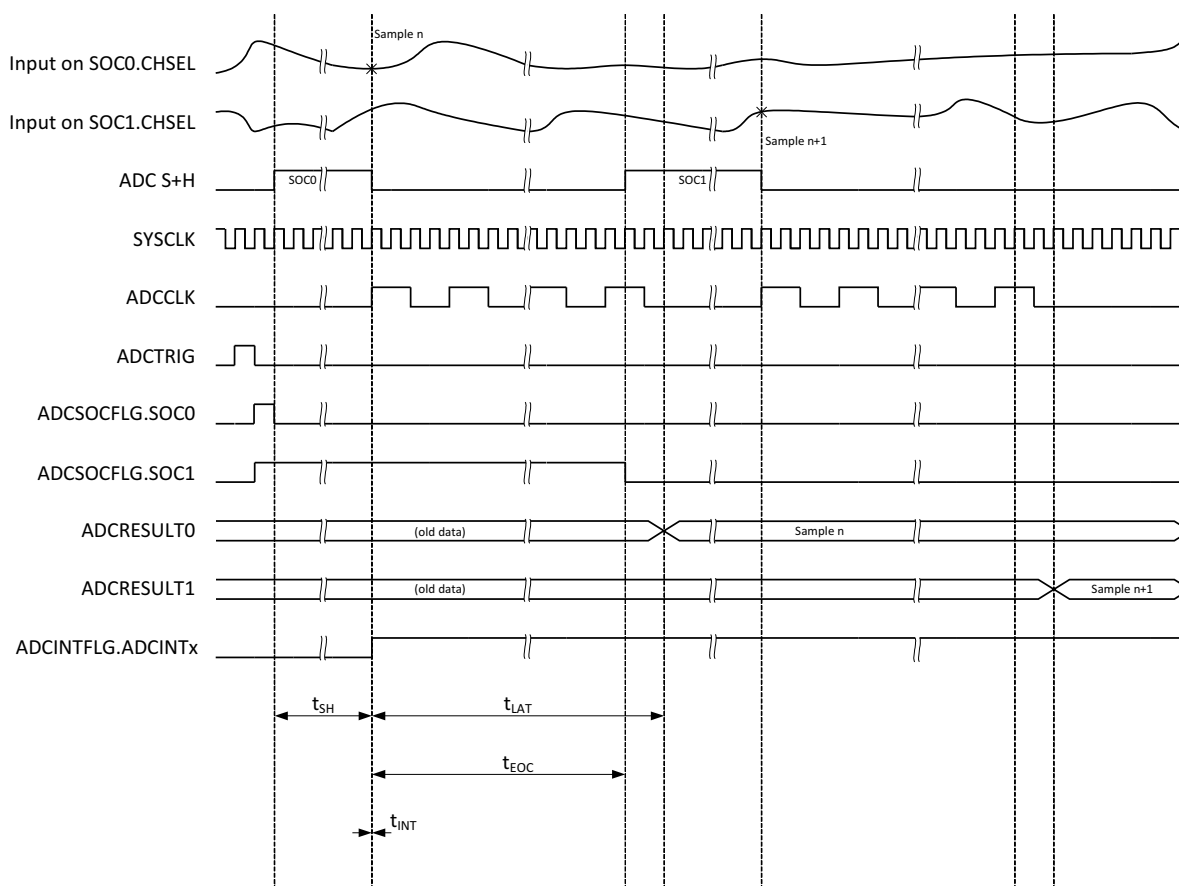
Figure 9-10. ADC Timings for 12-bit Mode in Early Interrupt Mode
