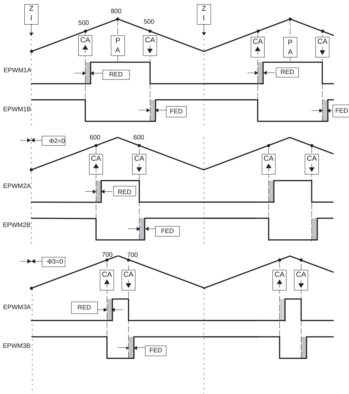
Figure 13-66. 3-Phase Inverter Waveforms for Figure 13-65 (Only One Inverter Shown)
