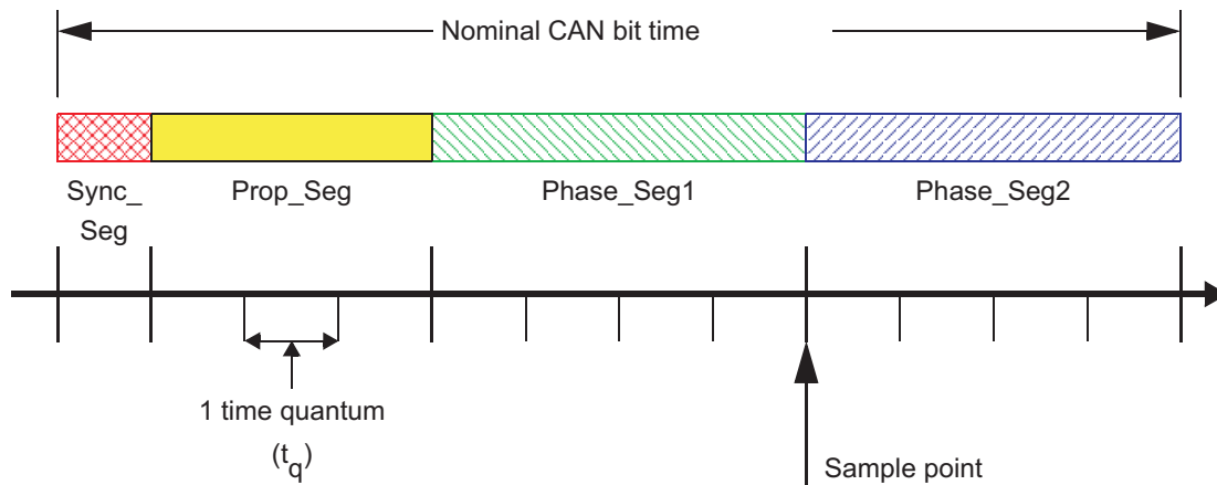
Figure 21-10. Bit Timing
