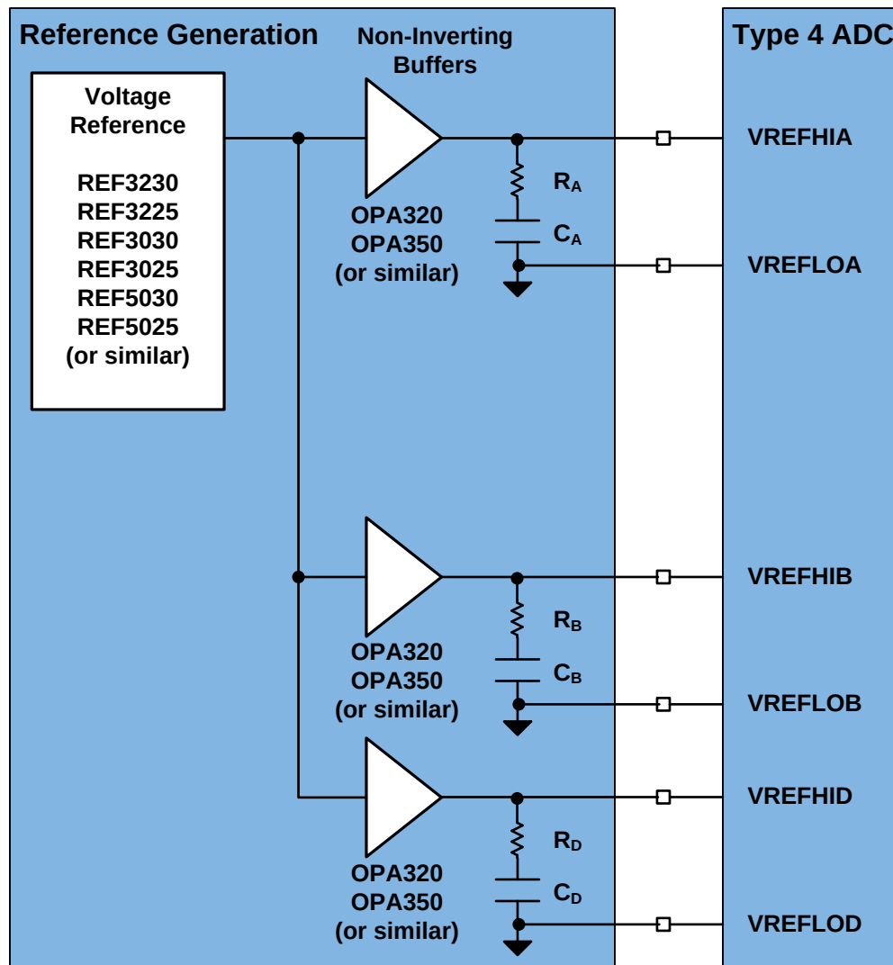
Figure 9-17. ADC Reference System
