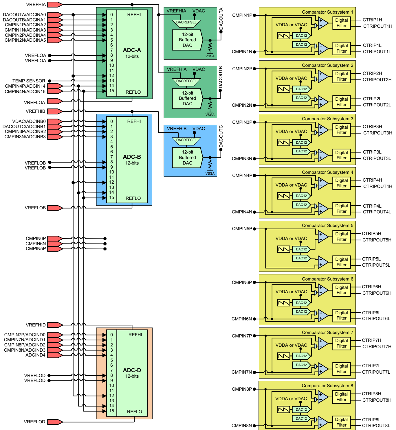
Figure 8-1. Analog Subsystem Block Diagram (176-Pin PTP)
