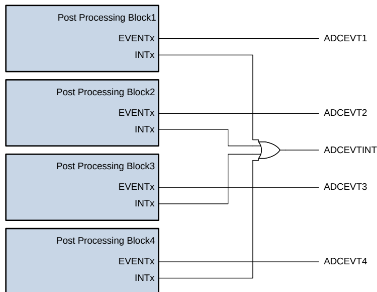
Figure 9-9. ADC PPB Interrupt Event
