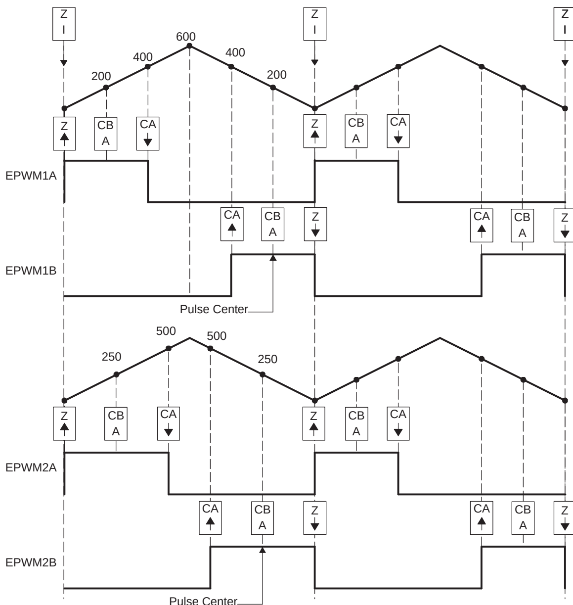
Figure 13-64. Half-H Bridge Waveforms for Figure 13-63 (Note: Here F_{PWM2} = F_{PWM1} )
