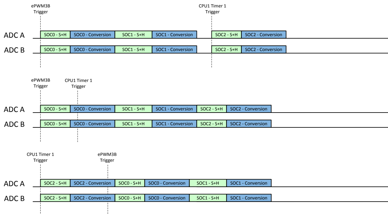
Figure 9-13. Example: Synchronous Operation with Multiple Trigger Sources
