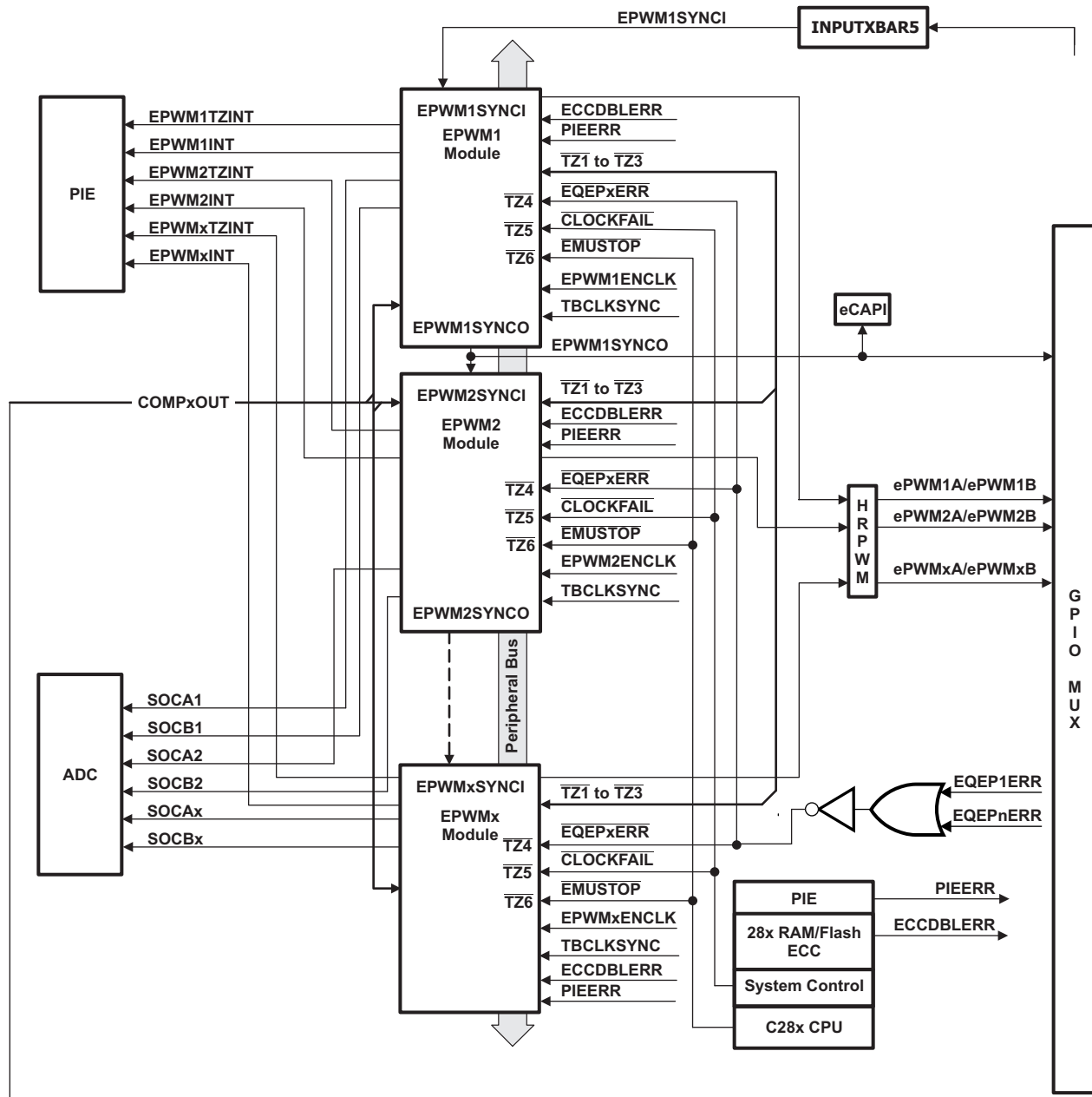
Figure 13-1. Multiple ePWM Modules
