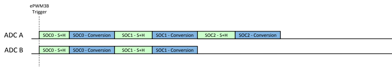
Figure 9-14. Example: Synchronous Operation with Uneven SOC Numbers
