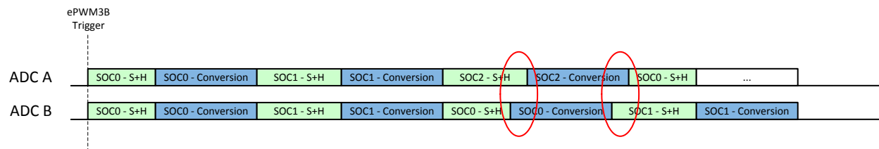
Figure 9-15. Example: Asynchronous Operation with Uneven SOC Numbers – Trigger Overflow
