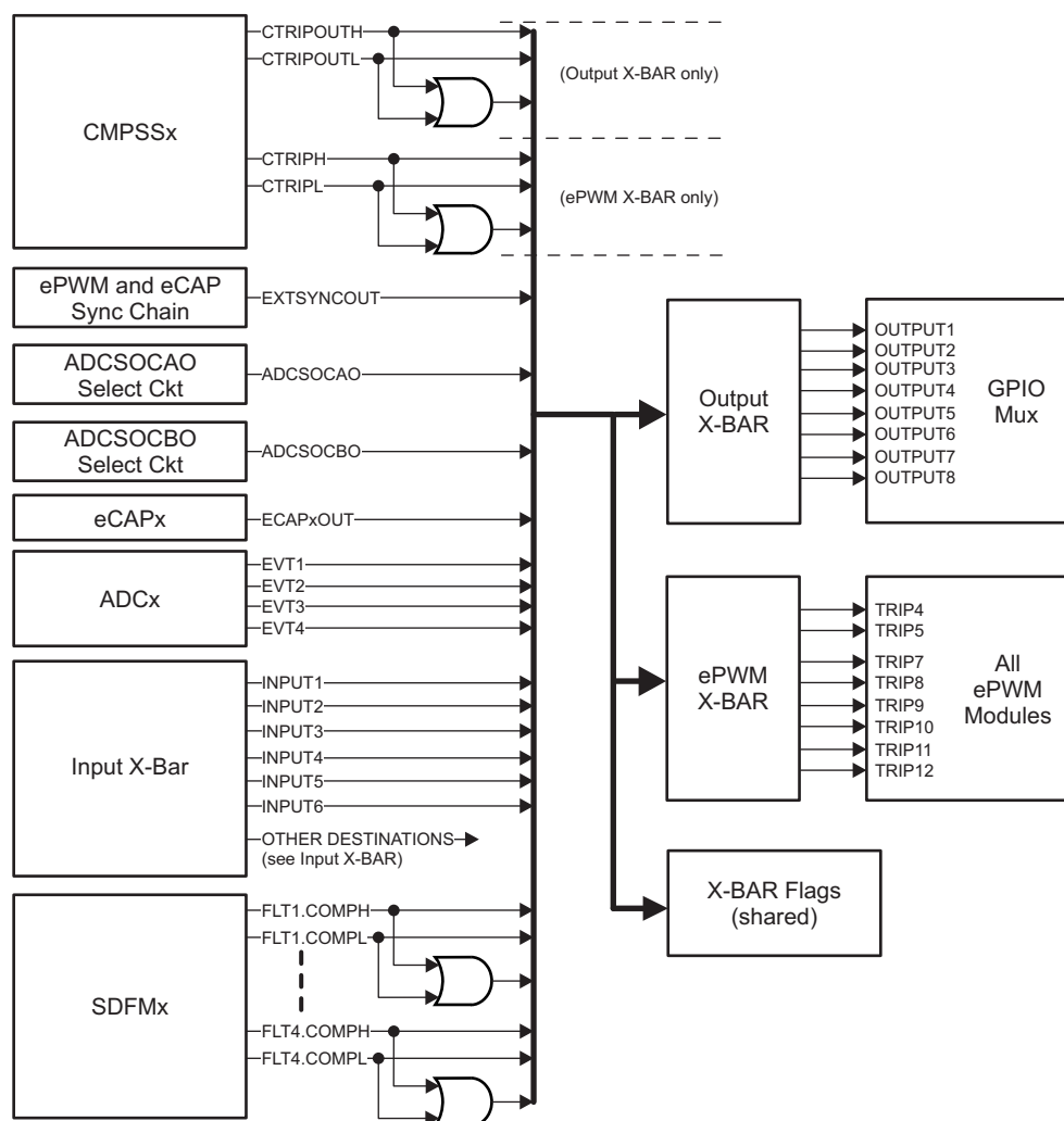
Figure 13-56. EPWM X-BAR
