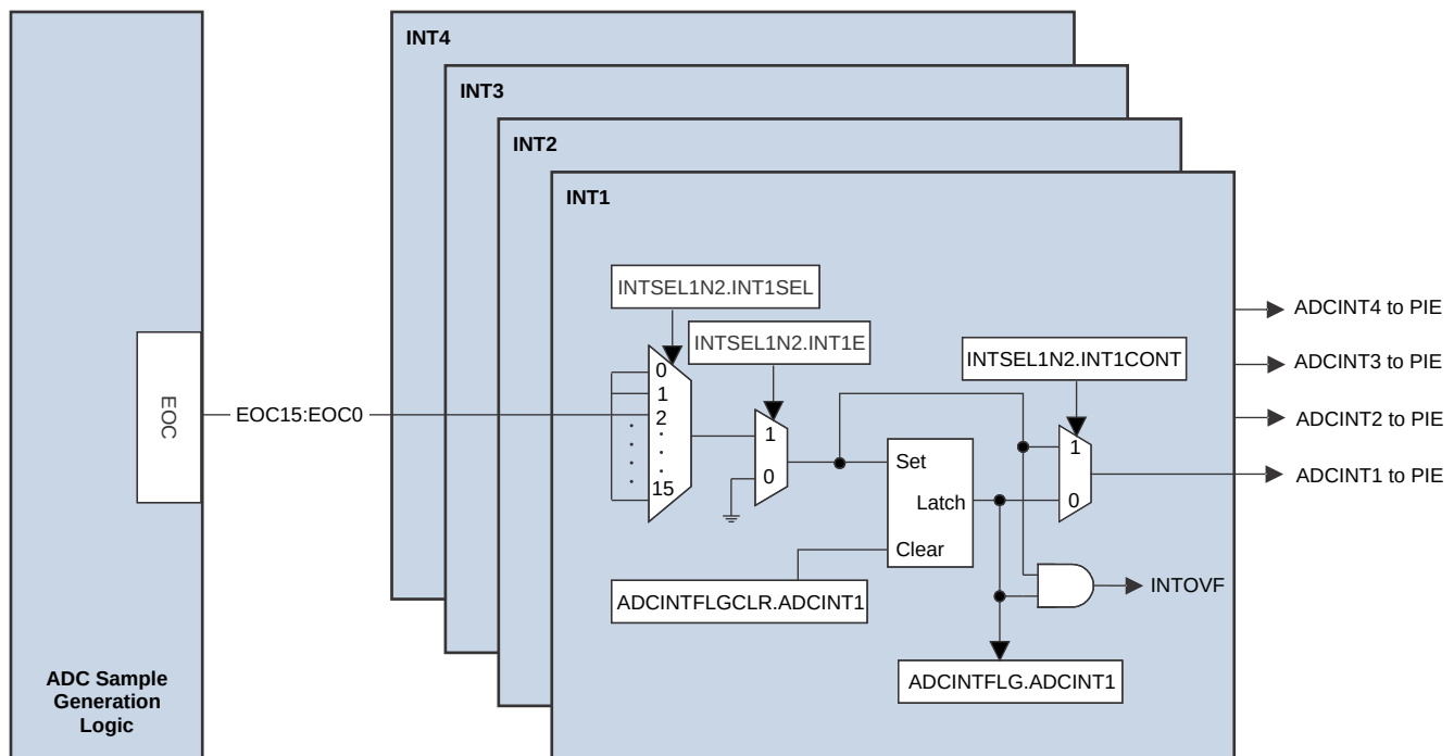
Figure 9-7. ADC EOC Interrupts
