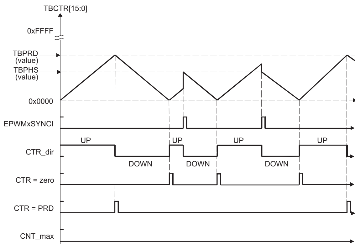
Figure 13-10. Time-Base Up-Down-Count Waveforms, TBCTL[PHSDIR = 0] Count Down On Synchronization Event
