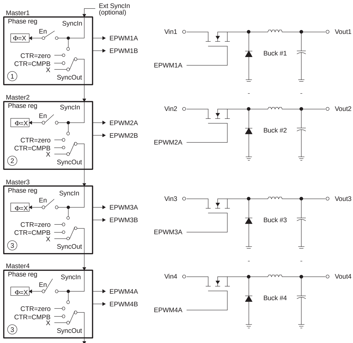
Figure 13-59. Control of Four Buck Stages. Here F_{PWM1} \neq F_{PWM2} \neq F_{PWM3} \neq F_{PWM4}
