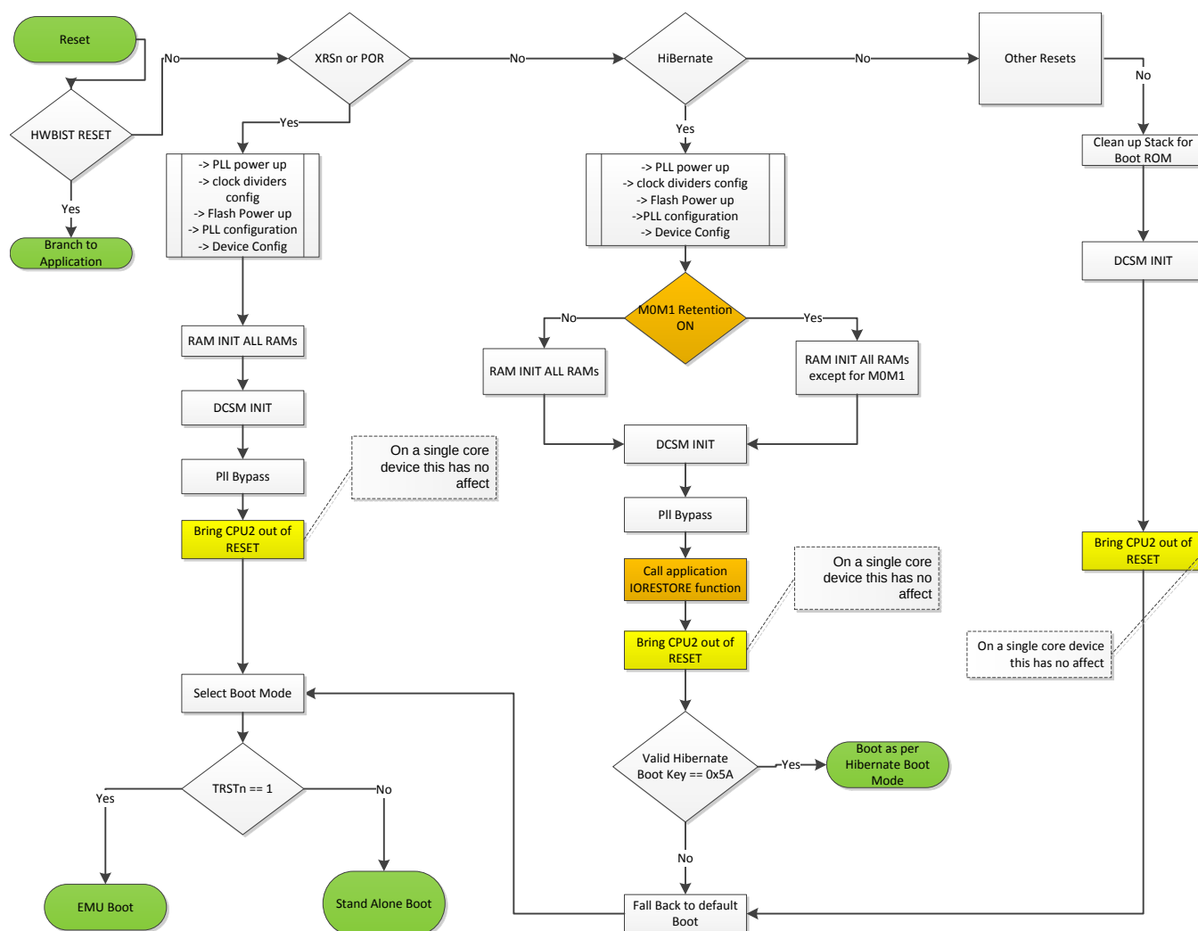
Figure 3-2. CPU1 Device Boot Flow
