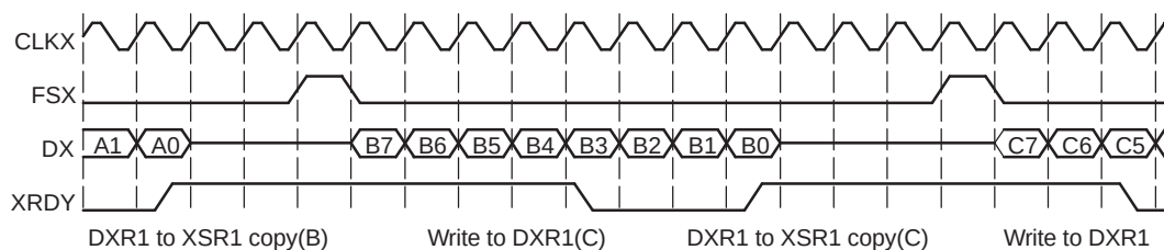
Figure 20-16. McBSP Transmission Signal Activity
