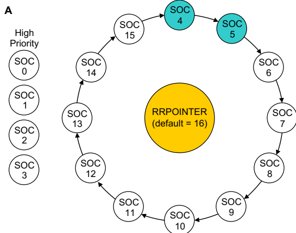
Figure 9-6. Burst Priority Example
