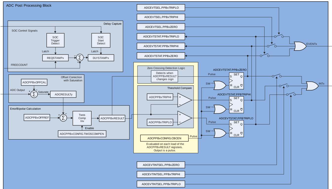
Figure 9-8. ADC PPB Block Diagram
