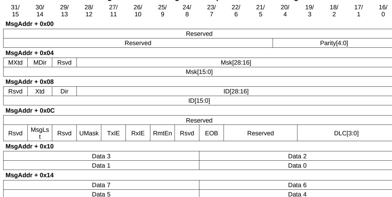
Figure 21-17. Message RAM Representation in Debug Mode
