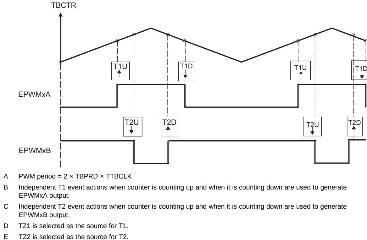
Figure 13-31. Up-Down-Count, PWM Waveform Generation Utilizing T1 and T2 Events
