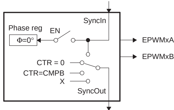
Figure 13-57. Simplified ePWM Module
