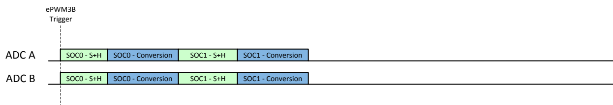
Figure 9-12. Example: Basic Synchronous Operation
