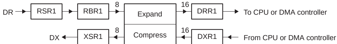
Figure 20-53. Companding Processes for Reception and for Transmission
