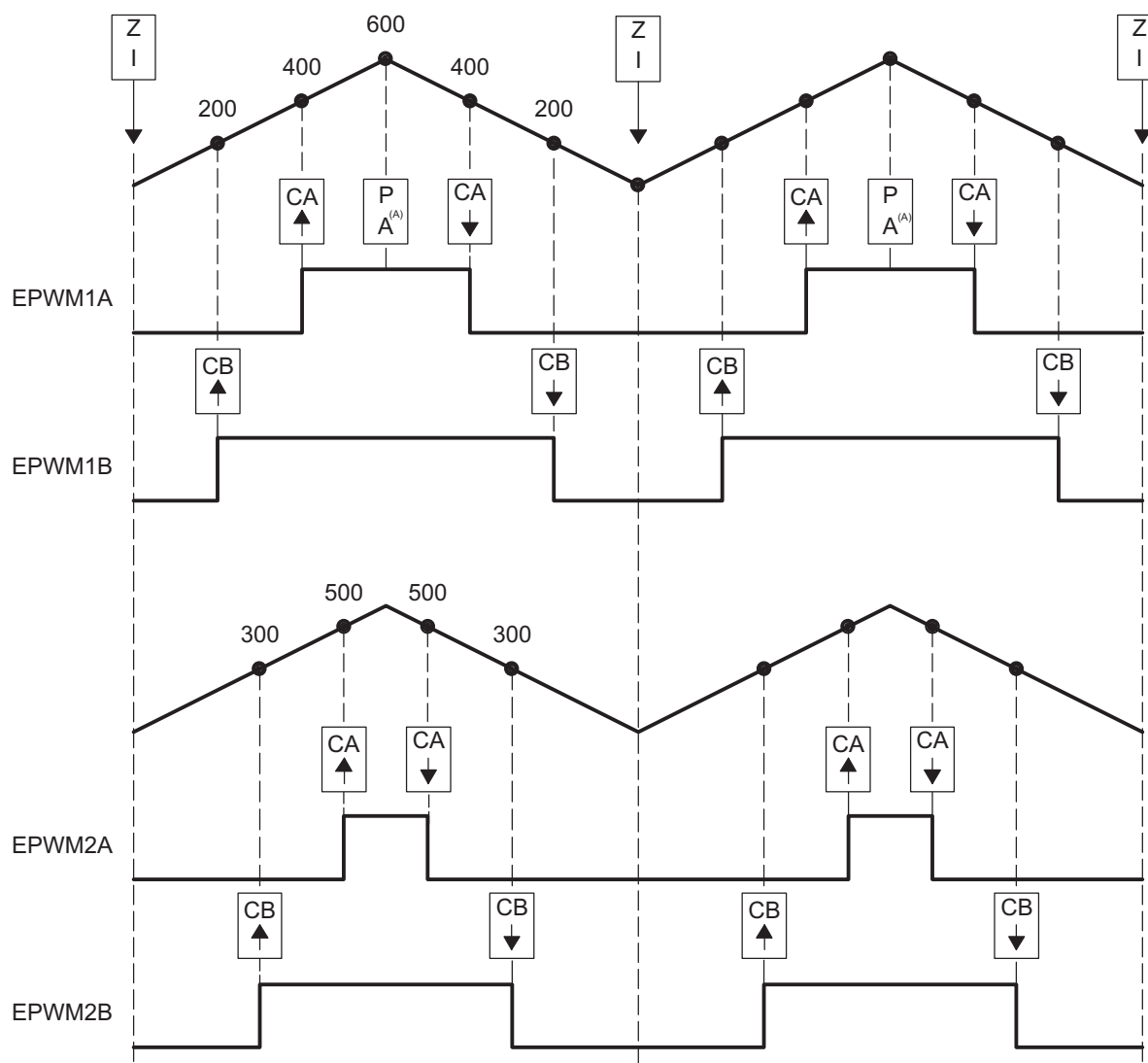
Figure 13-62. Buck Waveforms for Figure 13-61 (Note: F_{PWM2} = F_{PWM1} )
