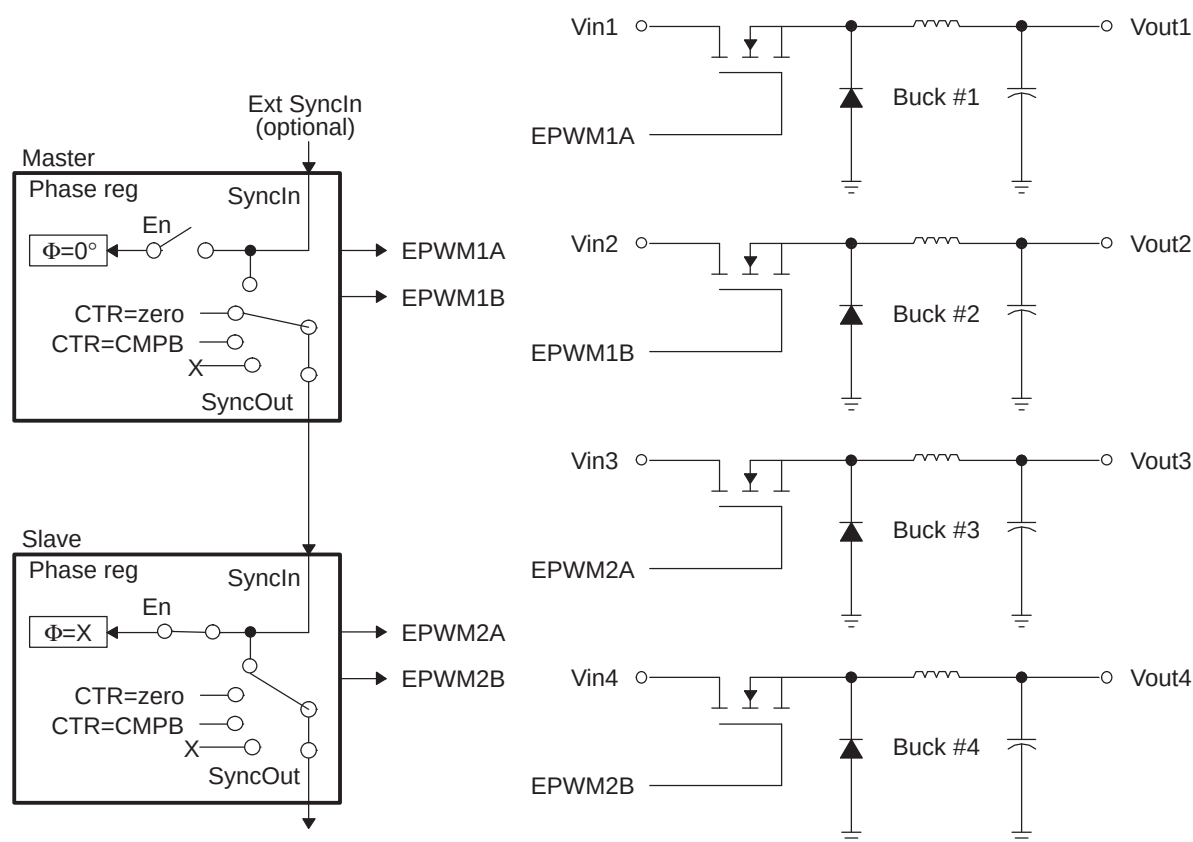
Figure 13-61. Control of Four Buck Stages. (Note: F_{PWM2} = N \times F_{PWM1} )
