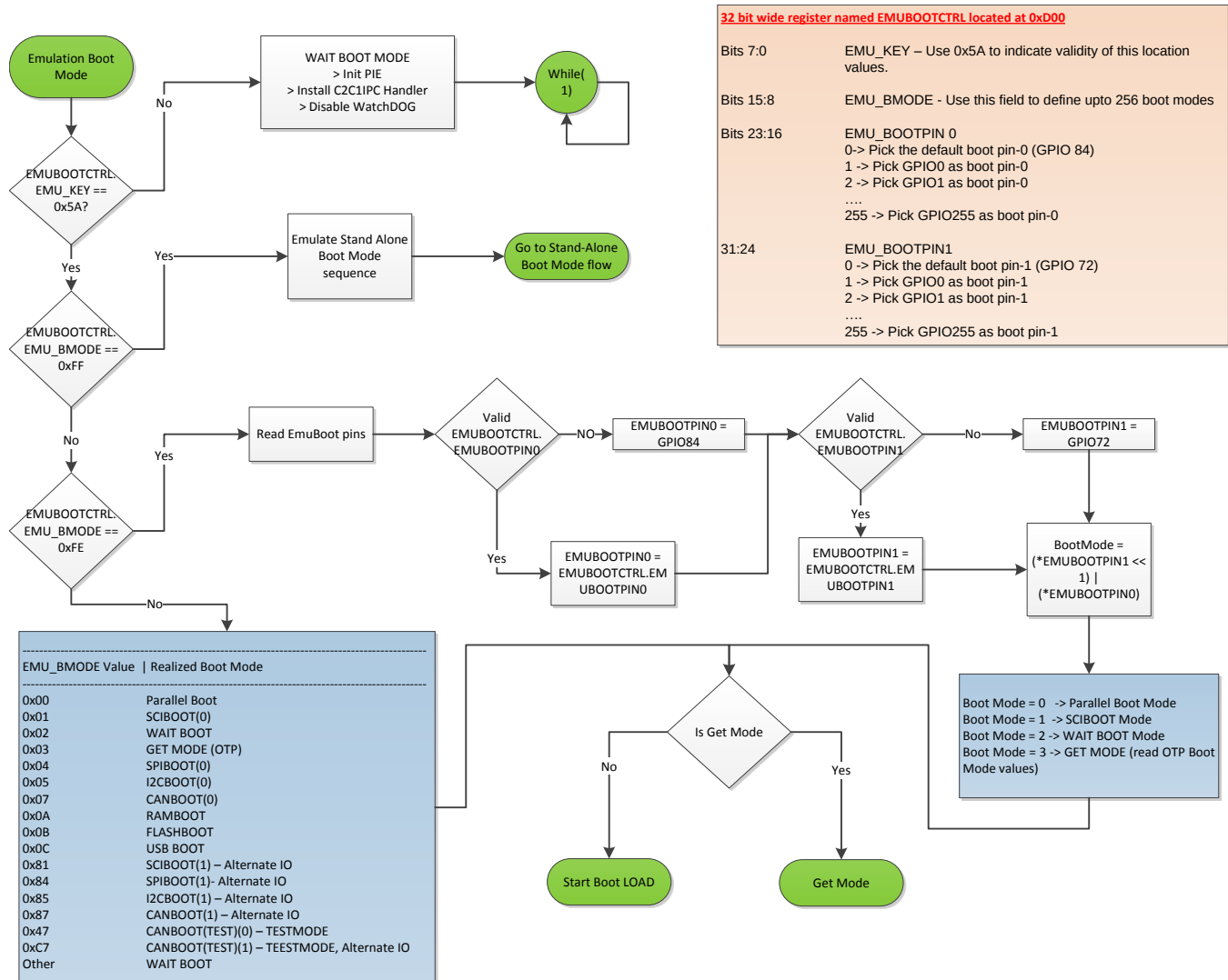
Figure 3-3. CPU1 Emulation Boot Flow
