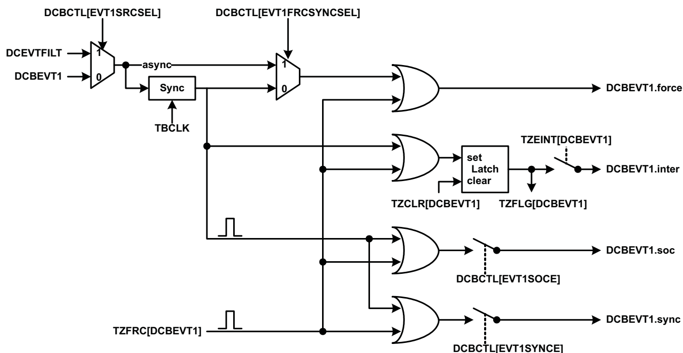
Figure 13-52. DCBEVT1 Event Triggering
