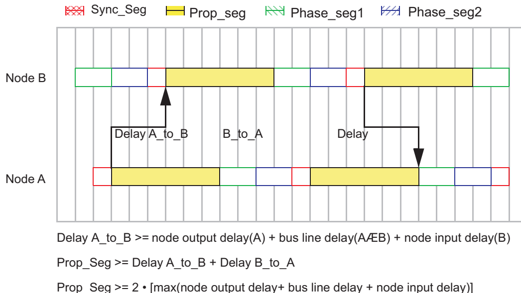
Figure 21-11. The Propagation Time Segment
