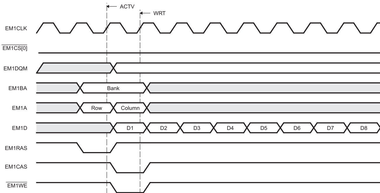
Figure 23-7. Timing Waveform for Basic SDRAM Write Operation
