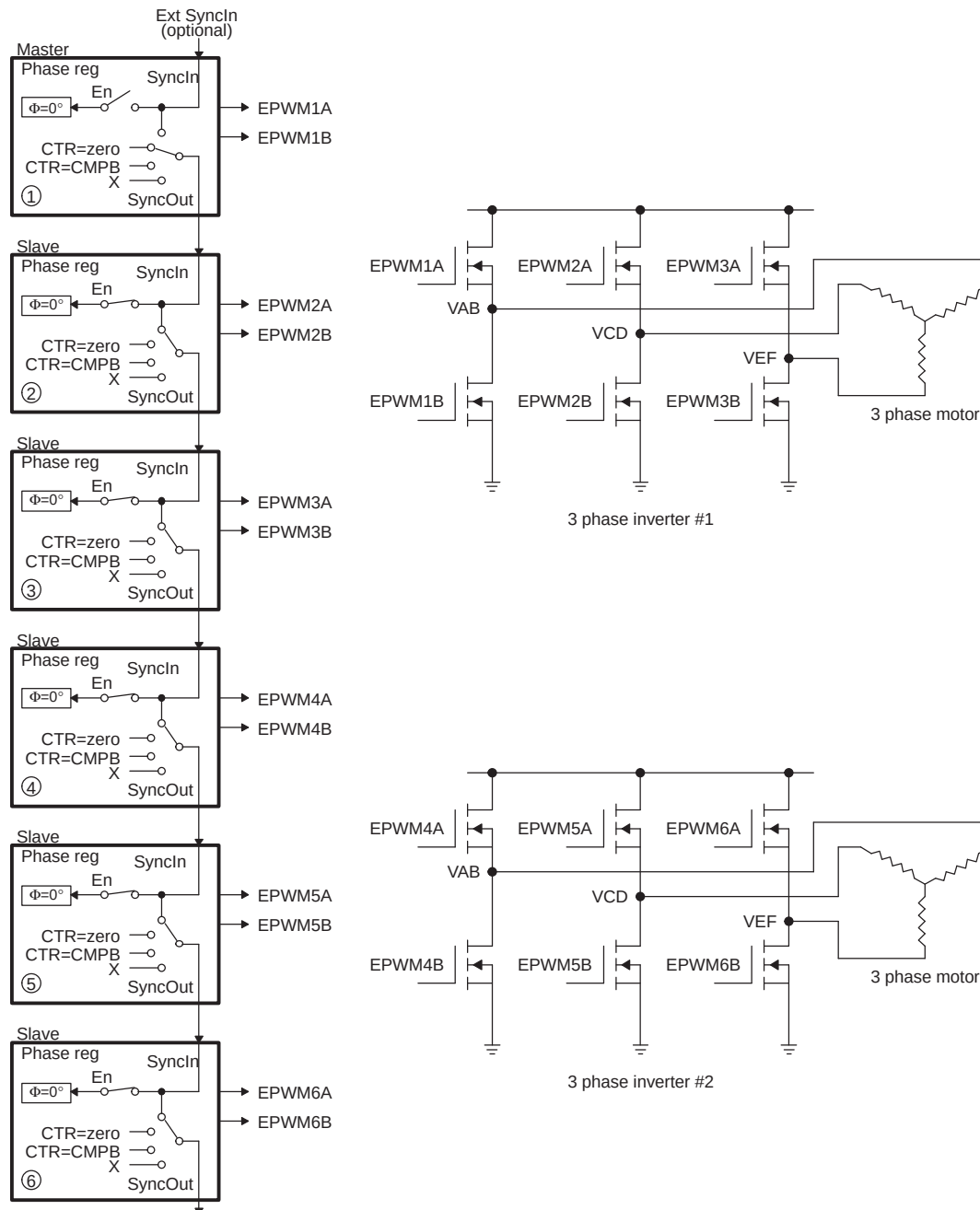
Figure 13-65. Control of Dual 3-Phase Inverter Stages as Is Commonly Used in Motor Control
