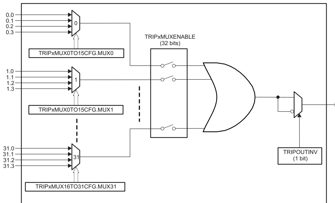
Figure 7-2. ePWM Architecture - Single Output
