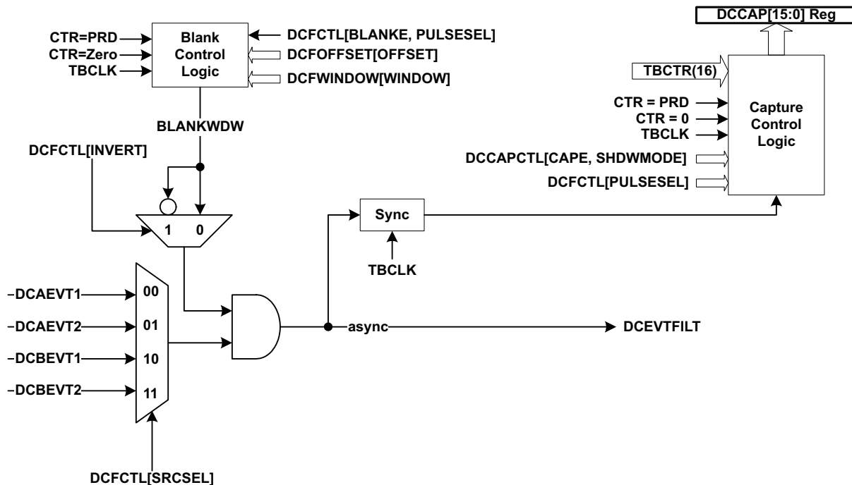
Figure 13-54. Event Filtering
