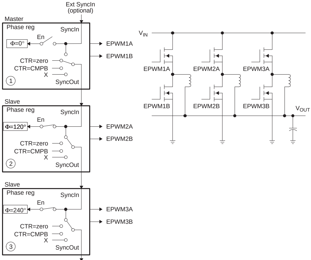
Figure 13-69. Control of a 3-Phase Interleaved DC/DC Converter
