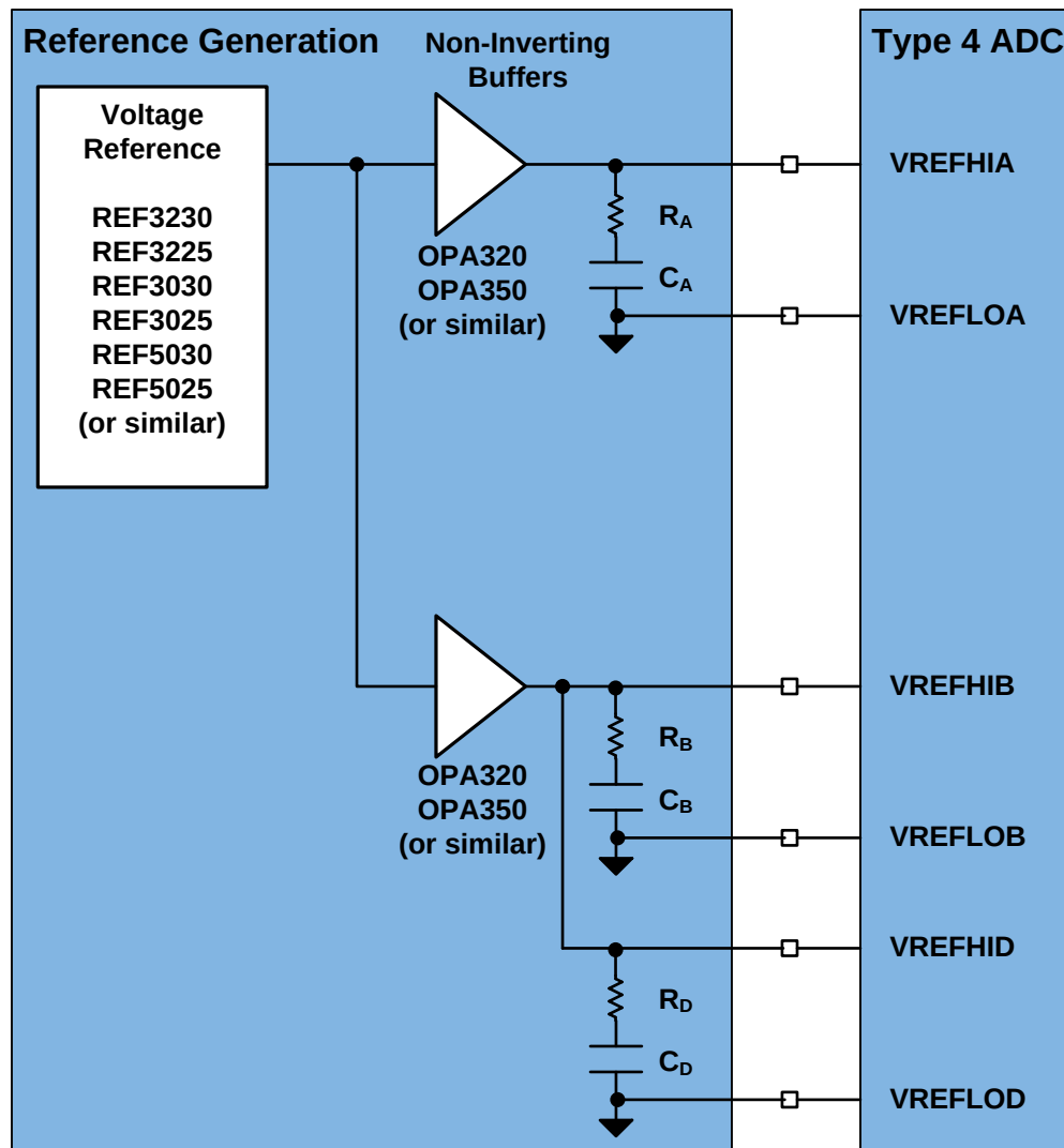
Figure 9-18. ADC Shared Reference System
