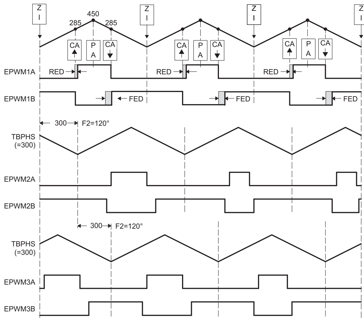
Figure 13-70. 3-Phase Interleaved DC/DC Converter Waveforms for Figure 13-69
