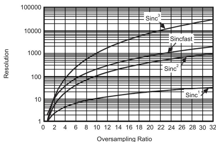
Figure 12-5. Comparator Filter Resolution
