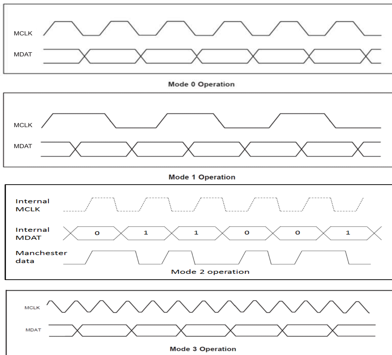
Figure 12-4. Operation Diagrams
