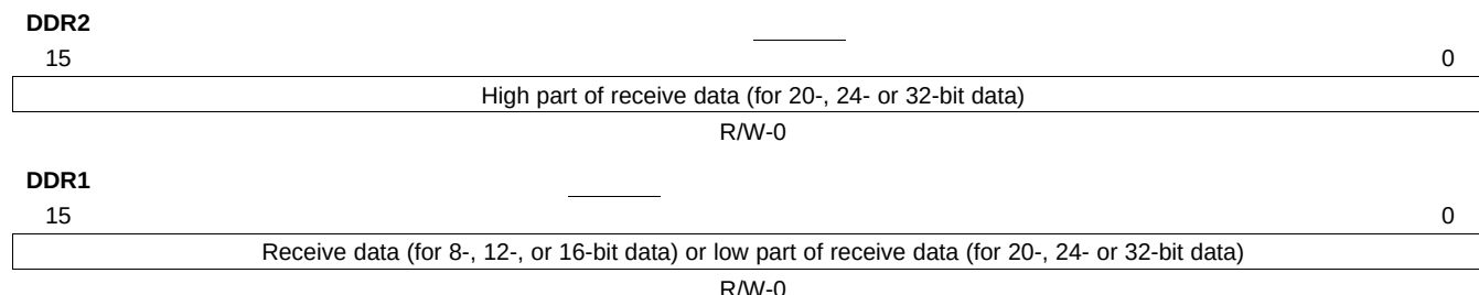
Figure 20-68. Data Receive Registers (DDR2 and DDR1)
