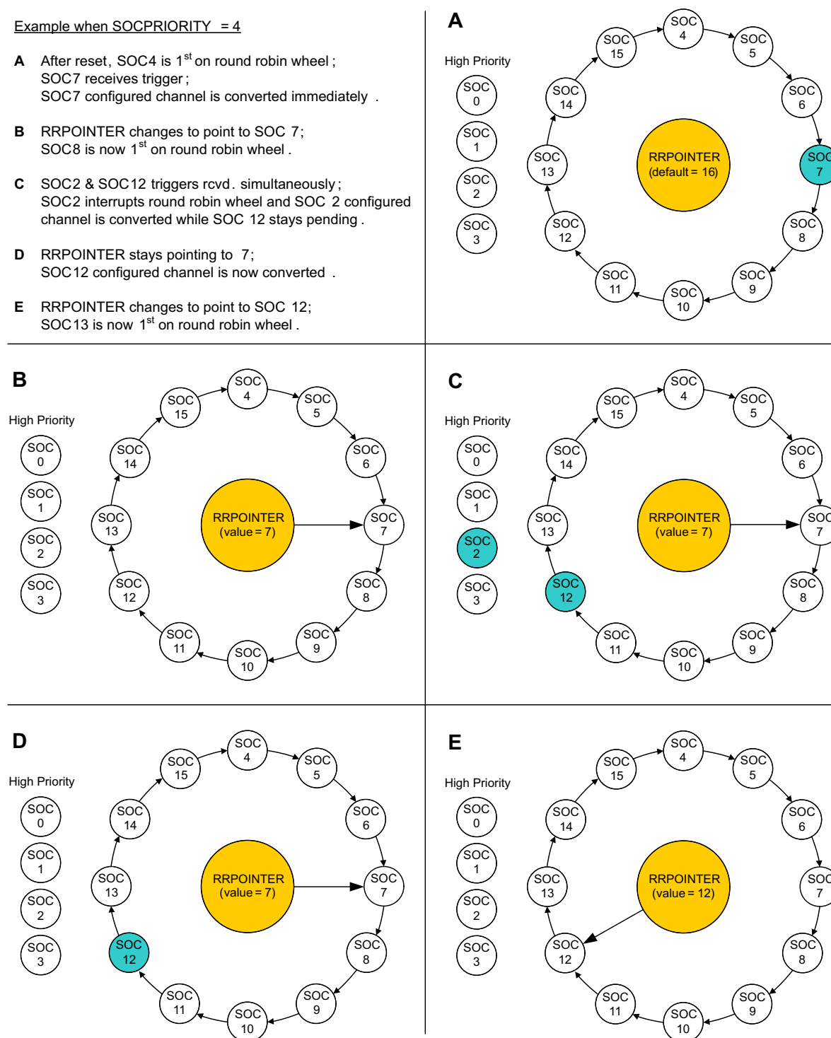
Figure 9-5. High Priority Example
