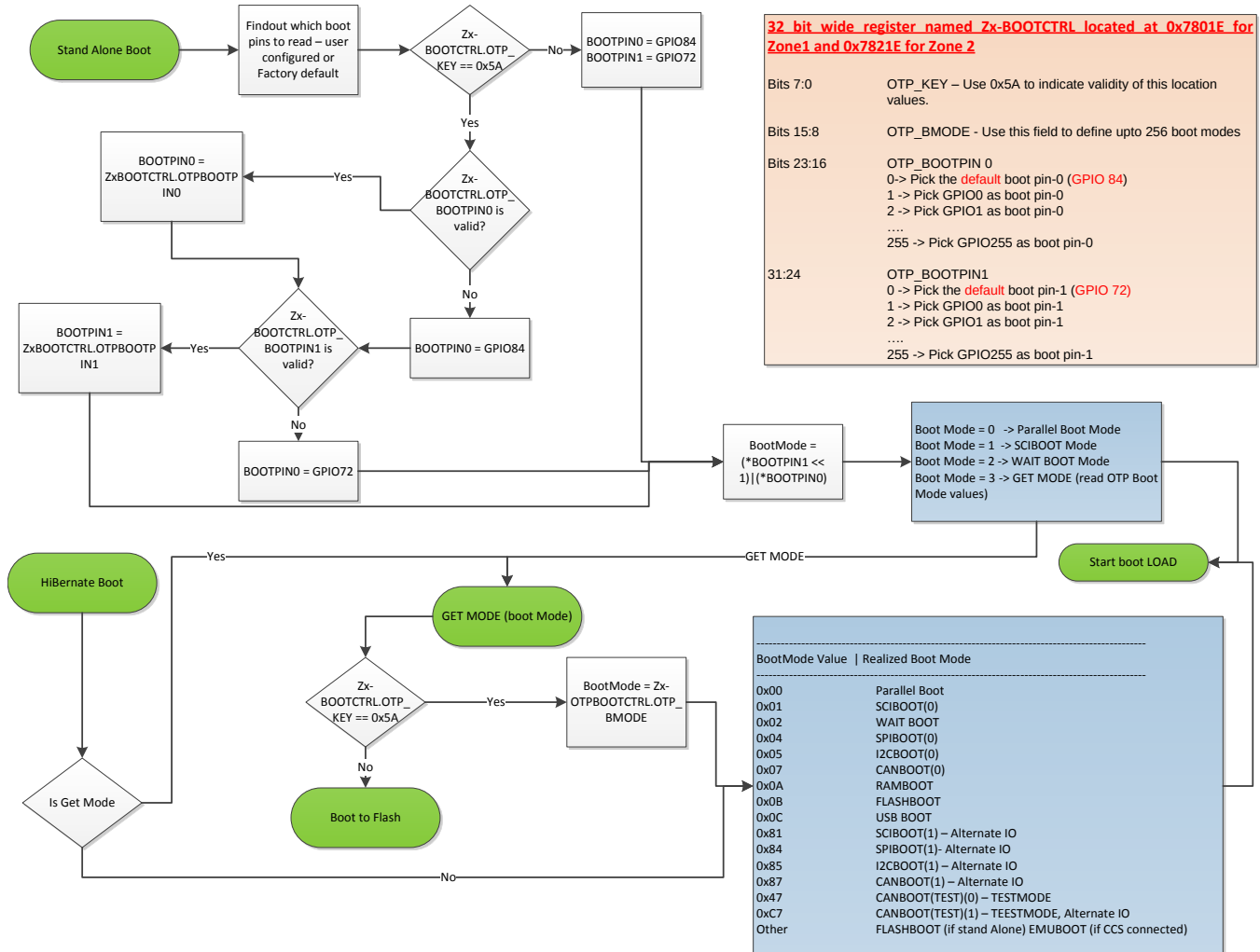
Figure 3-4. CPU1 Standalone and Hibernate Boot Flow
