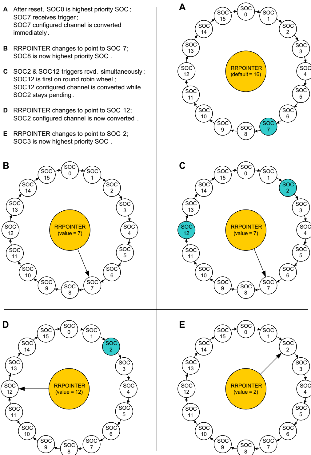
Figure 9-4. Round Robin Priority Example
