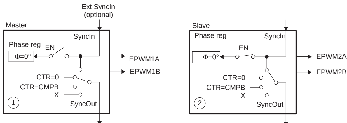
Figure 13-58. EPWM1 Configured as a Typical Master, EPWM2 Configured as a Slave
