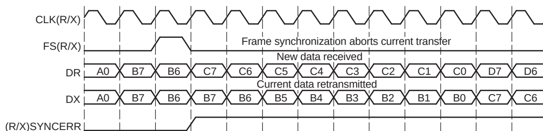
Figure 20-43. Unexpected Frame-Synchronization Pulse With (R/X)FIG = 0
