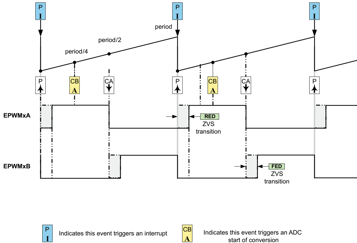
Figure 13-76. H-Bridge LLC Resonant Converter PWM Waveforms
