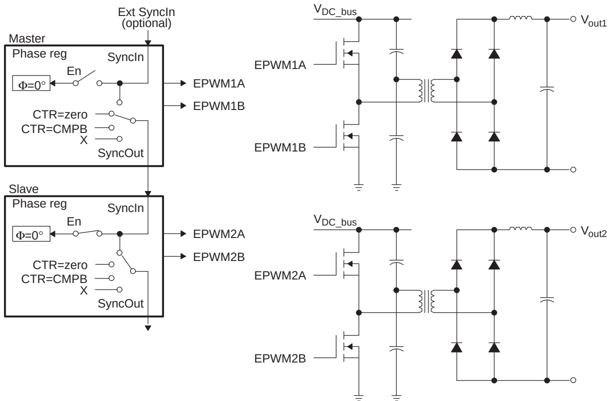
Figure 13-63. Control of Two Half-H Bridge Stages ( F_{PWM2} = N \times F_{PWM1} )
