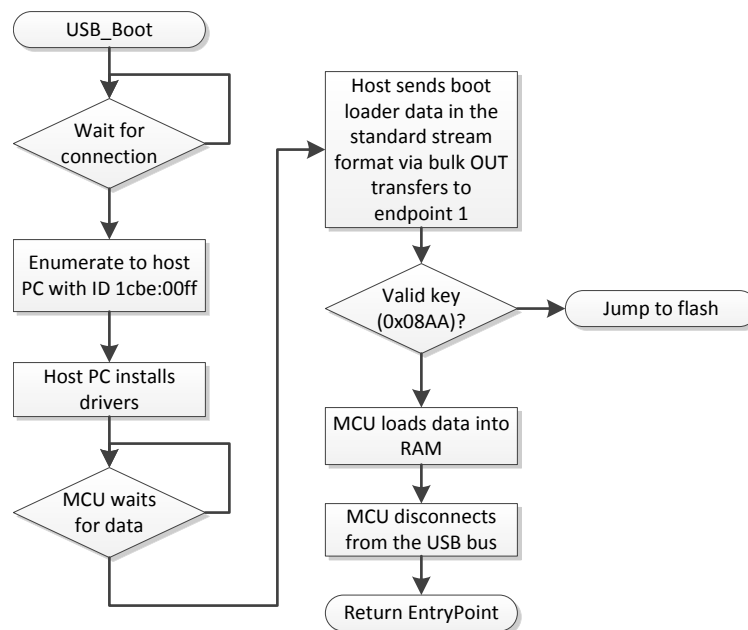
Figure 3-19. USB Boot Flow
